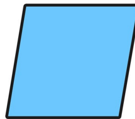
parallelogram
