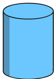
cylinder
