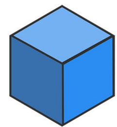
cube
