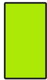
rectangle
